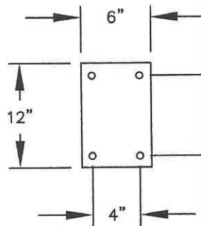
PEDESTAL BASE BOLT PATTERN
