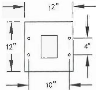
PEDESTAL_BASE BOLT_PATTERN
