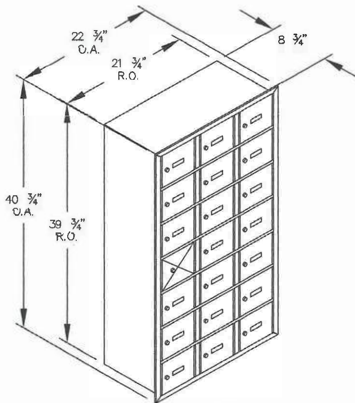
Recessed Mt., 7H x 3W Configuration (21A / 20A Utilized for Storage)
